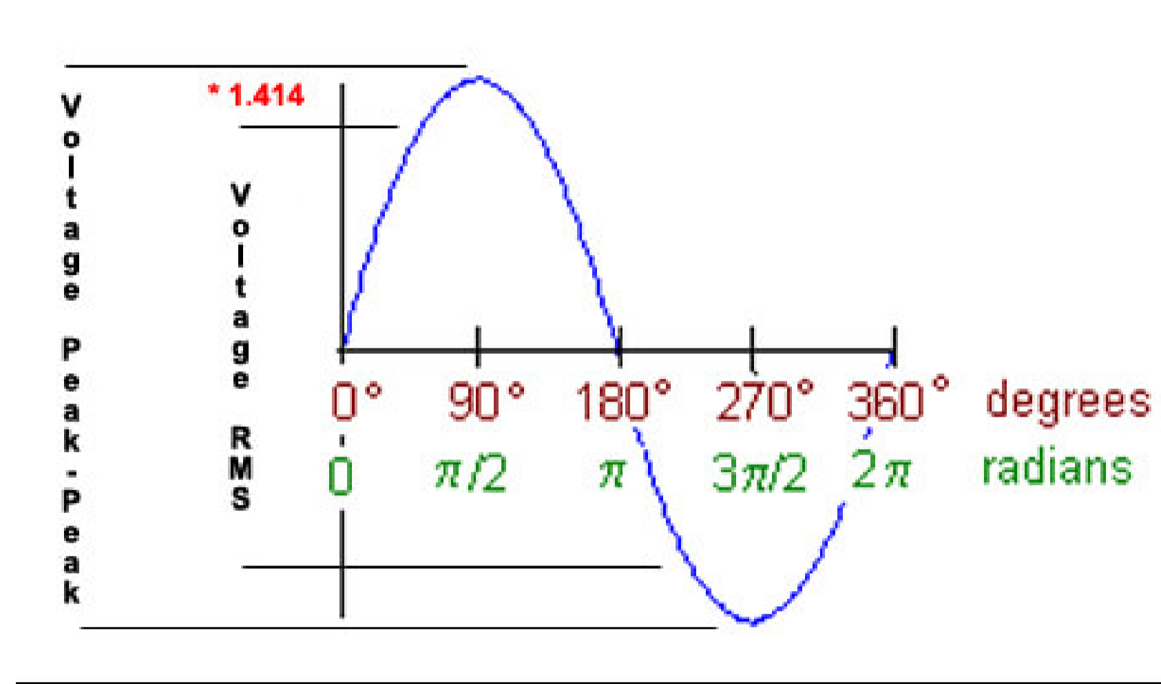
Figure 1.0: Peak vs. RMS Measurement of a Sinusoid
