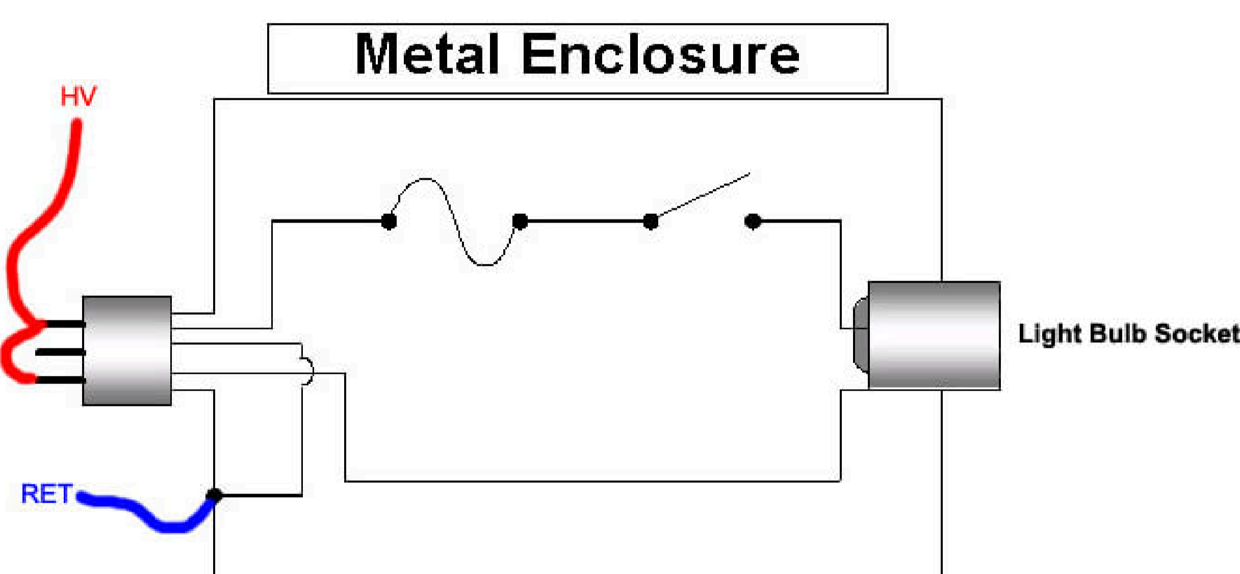
Figure 2.0: Hipot Test Connection Diagram
