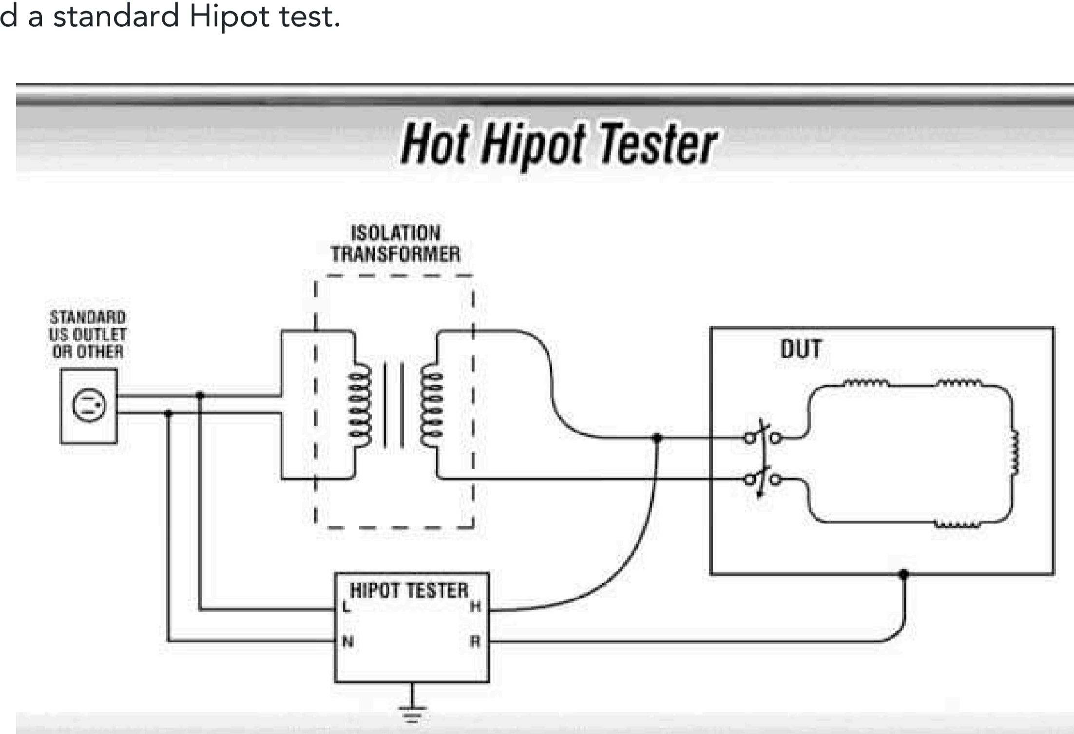
Figure 3.0: Hot Hipot Test Connection Diagram
